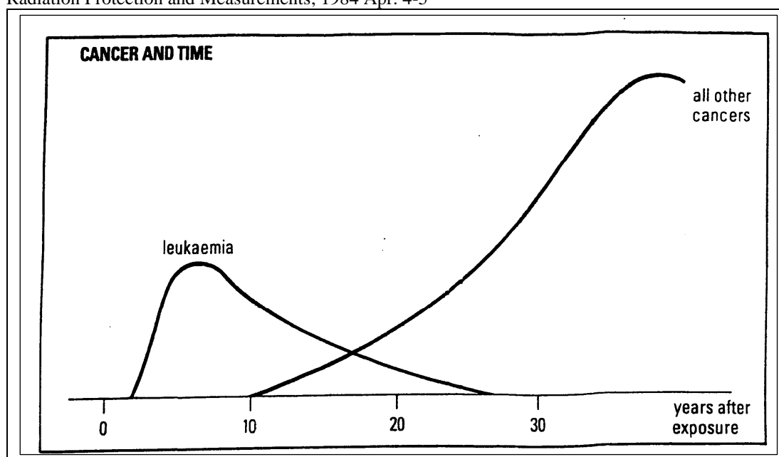
Fig. 4. – Curve showing the appearance of leukemia and solid cancers over time, after a single exposure to radiation (1 REM) of sufficient dose to cause a tumor. Figure taken from: Radiation: doses, effects, risks , United Nations Scientific Environment Programme; 1985, p. 54. In: Sinclair WK, editor. Twentieth Annual Meeting of the National Council on Radiation Protection and Measurements; 1984 Apr. 4-5
